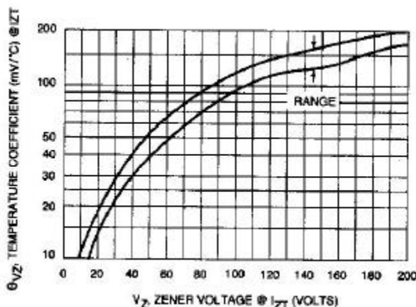
Fig. 6-UNITS 10 TO 200 VOLTS
