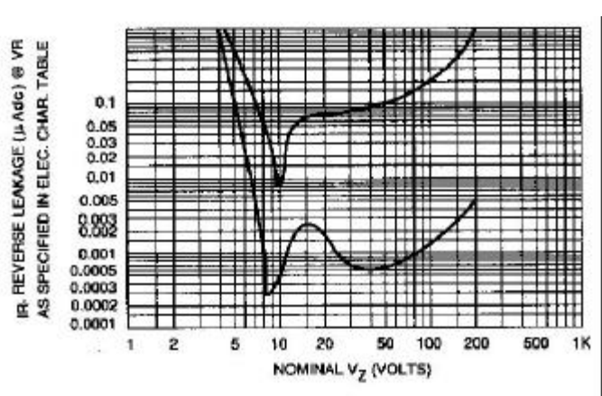
Fig. 4-TYPICAL REVERSE LEAKAGE
